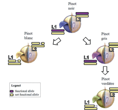
Fig. 4. Model of the formation of Pinot blanc, Pinot gris, and Pinot verdâtre from Pinot noir. A scheme represents ...
